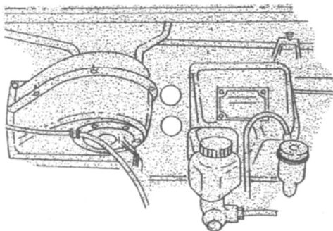
DETAIL A FIREWALL HOLES FOR P-1800
