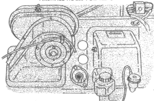
DETAIL B FIREWALL HOLES FOR 122-S
